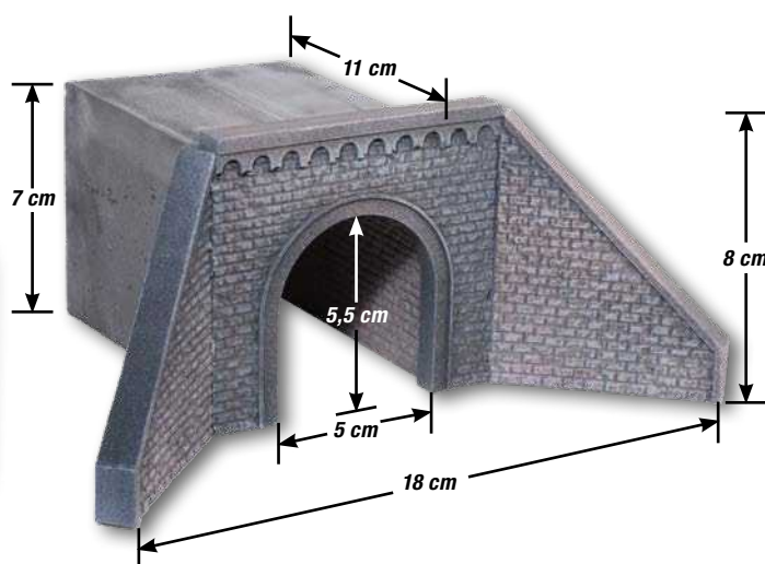
H0 58292 Underpass 1 portal, 2 wing walls, 1 pipe
