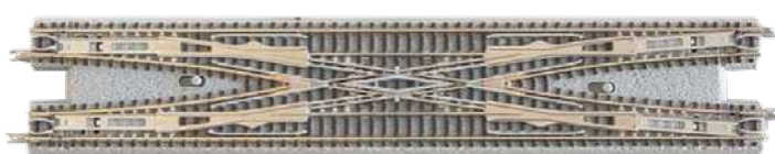
7297078 (R078) Double Crossover 220 mm, 25 mm track distance (1 piece)
