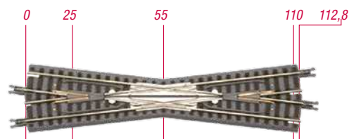
7297020 (R020) Crossing 13° , 112.8 mm, with 2 x Adjustment Track 53.6 mm (1 piece)
