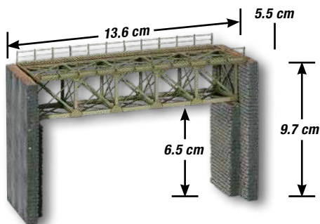
H0e H0m 67038 Steel Bridge with bridgeheads. This bridge is not combinable with other Laser-Cut bridges.
