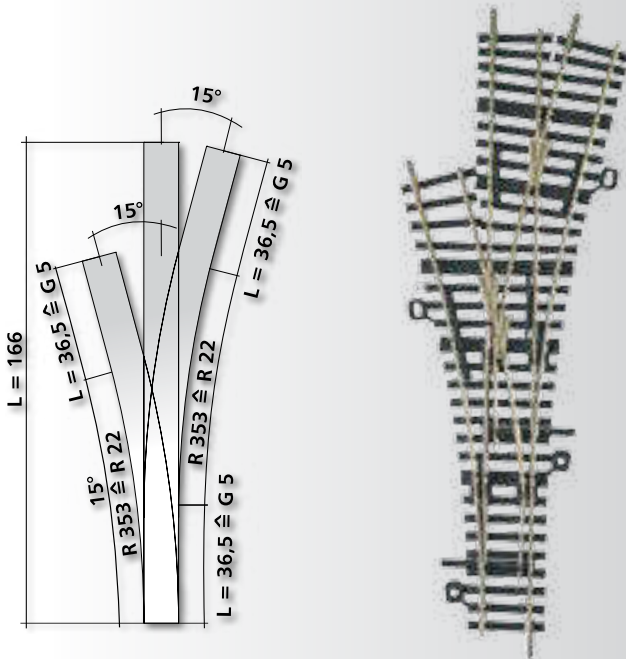
DWW, 2 x 15°, 166 mm asymmetrisch / asymmetrical Art.-Nr: 83230
