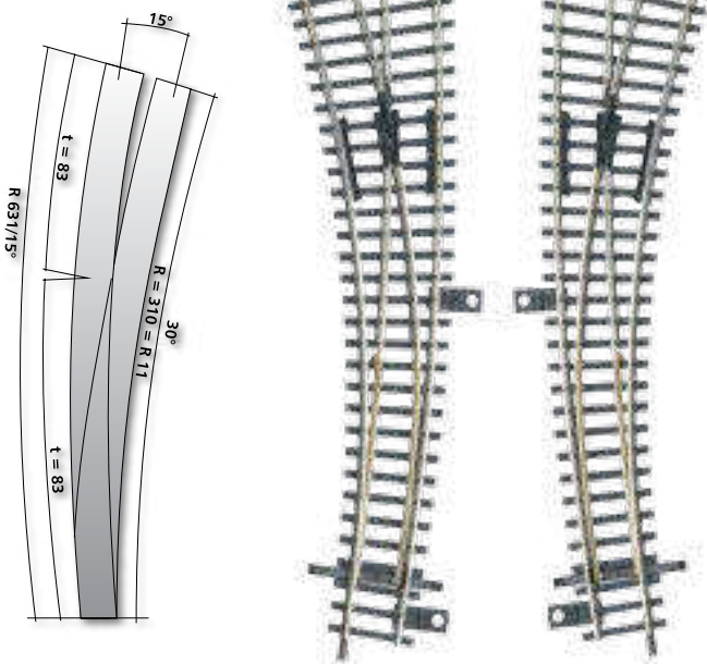
IBW, links IBW, left points Art.-Nr: 83362
